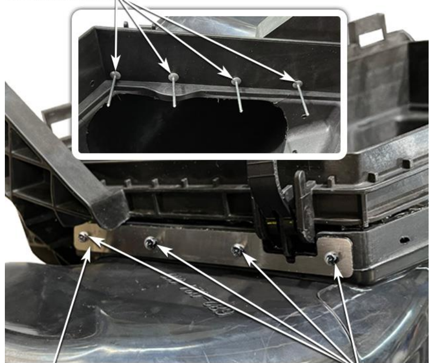
Install Plate
