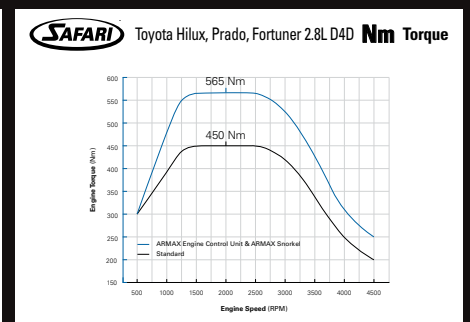
Results at engine flywheel
