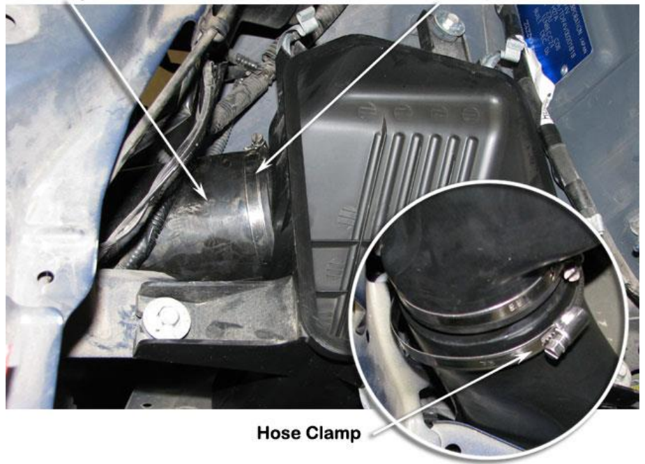
Air Entry Hose
